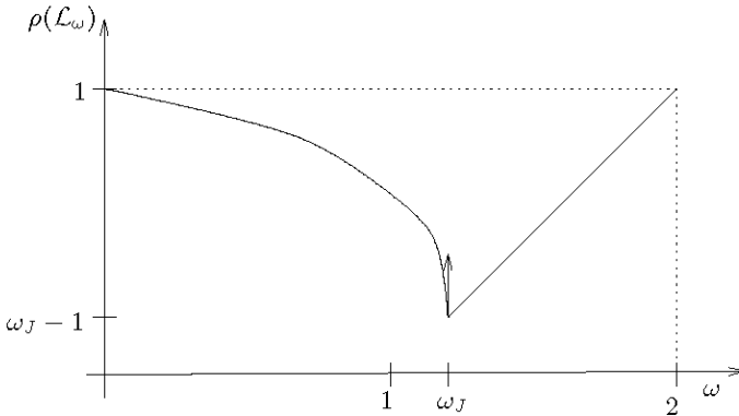
Figure 9.1. \rho(\mathcal{L}_\omega) in the tridiagonal case.
